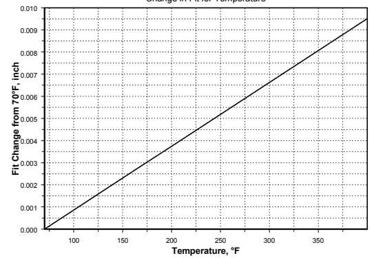
150R1230 Roper 1-1/2" 1/2 3 Stage Power Section Change in Fit for Temperature
